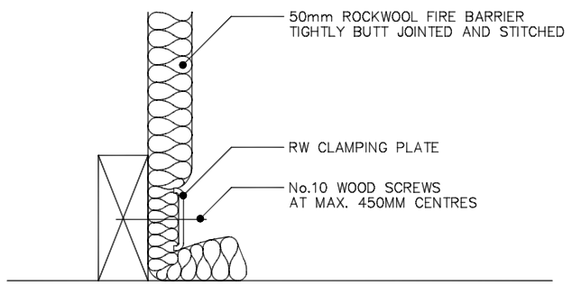
ROCKWOOL FIRE BARRIER Fire Stopping: (Roof) 1/2 Hour Cavity Barrier In Roof Void In Line With Rafter (Min. 50mm Wide Rafters) FB05
