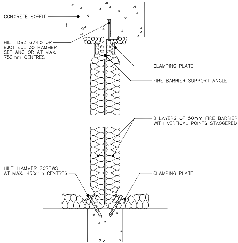
ROCKWOOL FIRE BARRIER Fire Stopping: (Roof) 1 Hour Fire Barrier In Roof Void FB02
